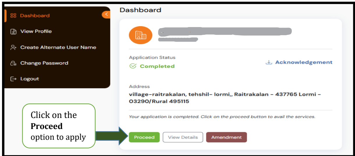
Figure 4.1: Dashboard
